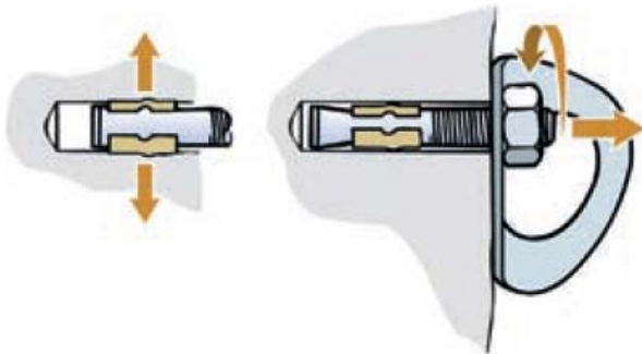
Abb. 2 Expressanker
